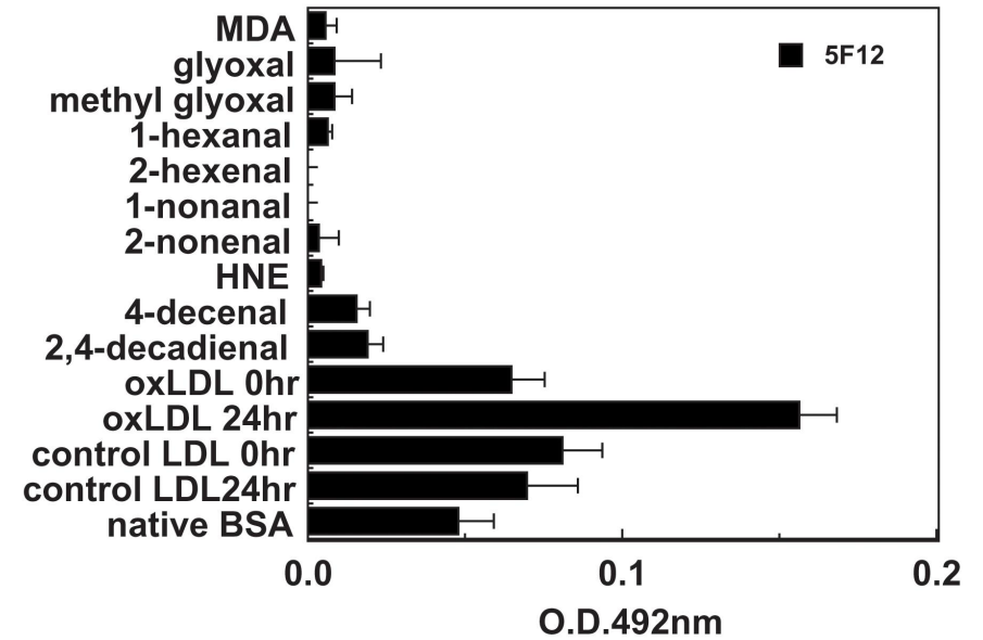
Cross reactivity
